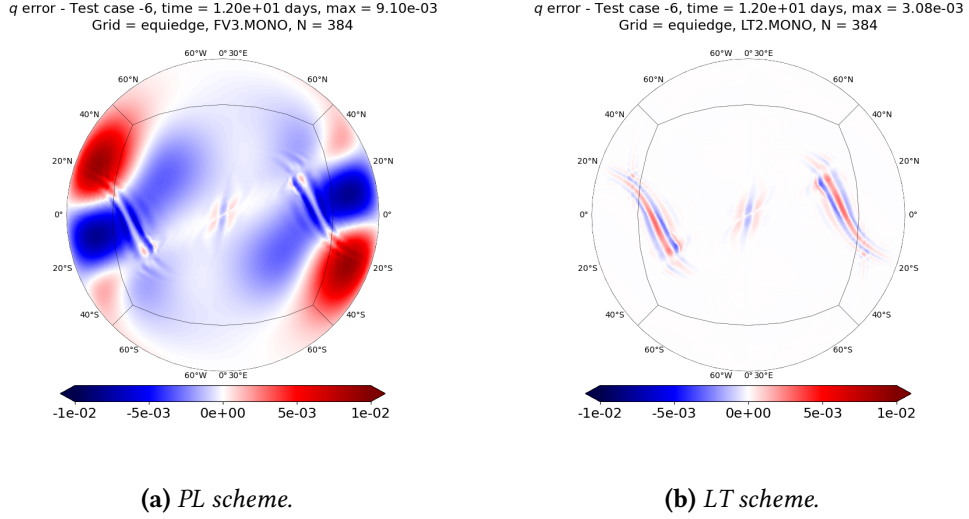
Figure 5.22: Advection experiment errors using the two Gaussian hills (IC4, Table 5.2) and the divergent wind (VF3, Table 5.3) after 12 days, using the monotonic scheme (MONO) with PL (left) and LT schemes (right) on the equi-edge grid ( g_0 ) with N = 384 .
