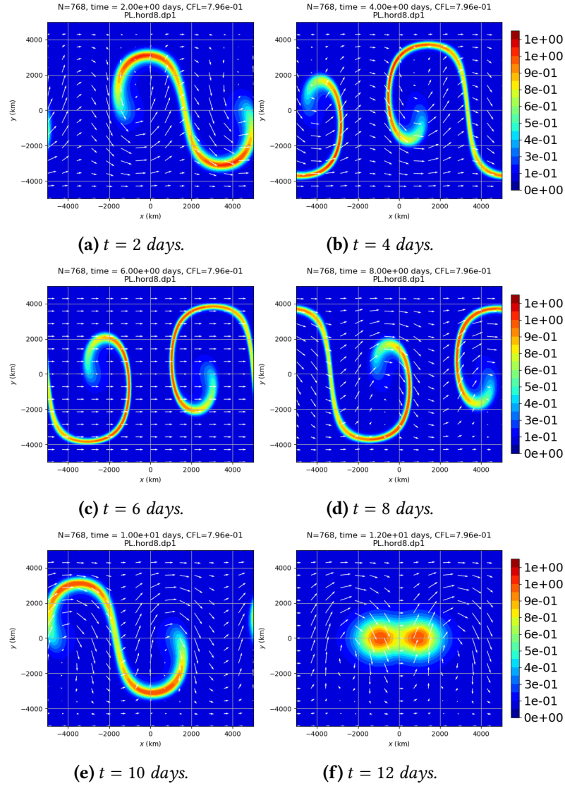
Figure 3.6: Linear advection experiment using the velocity from Equation (3.32), a CFL number equal to 0.79, N = 768 cells, and the IC is given by Equation (3.31). These figures show the advected profile at 2 (3.6a), 4 (3.6b), 6 (3.6c), 8 (3.6d), 10 (3.6e), and 12 (3.6f) days. The white arrows illustrate the velocity field. We are using the PL-DP1-MONO scheme, where MONO is the monotonic PPM.
