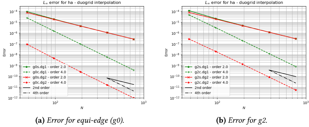
Figure 4.10: Error for the duo-grid interpolation of the scalar field of (4.51) for the equi-edge grid (g0, left) and the equiangular grid (g2, right). Dashed lines use the cube midpoint formulation, while solid lines use the spherical midpoint formulation. Green lines represent dg1, and red lines represent dg2.
