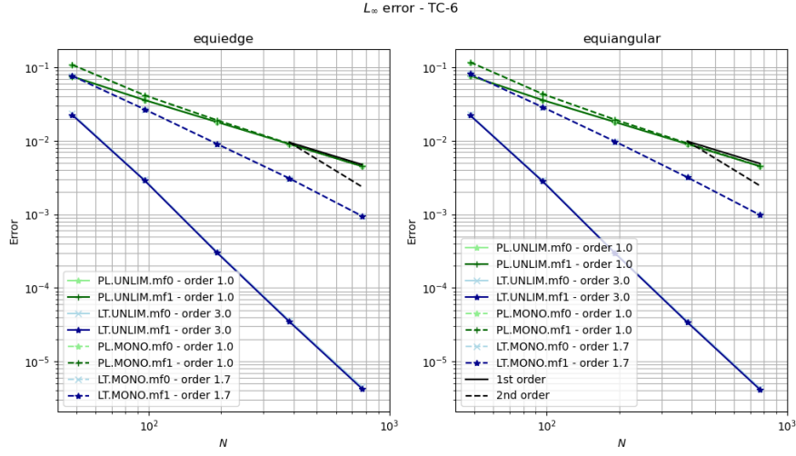
Figure 5.24: L_\infty error convergence for the advection on the sphere test using the two Gaussian hills (IC4, Table 5.2) and the divergent wind (VF3, Table 5.3) on the equi-edge grid (g0, left) and on the equiangular grid (g2, right) after 12 days. Blue lines indicate the use of the LT scheme, while green lines represent the PL scheme. Solid lines represent the results with the unlimited PPM (UNLIM) scheme, whereas dashed lines represent the results with the monotonic PPM (MONO). Light colors show the result without mass fixer (mf0), whereas dark colors show the results with flux averaging (mf1).
