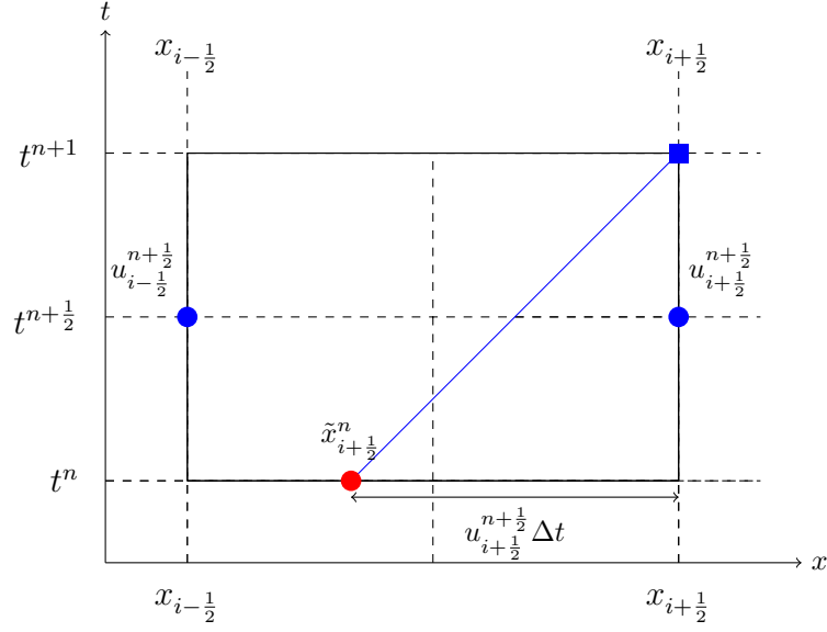
Figure 2.4: Illustration of the scheme DP1 for computing the departure point at time level n emanating from x_{i+\frac{1}{2}} (blue square) at time level n+1 , assuming u_{i+\frac{1}{2}}^{n+\frac{1}{2}} > 0 . The winds used are denoted by blue circles. The estimated departure point \tilde{x}_{i+\frac{1}{2}}^n is illustrated by a red circle.
